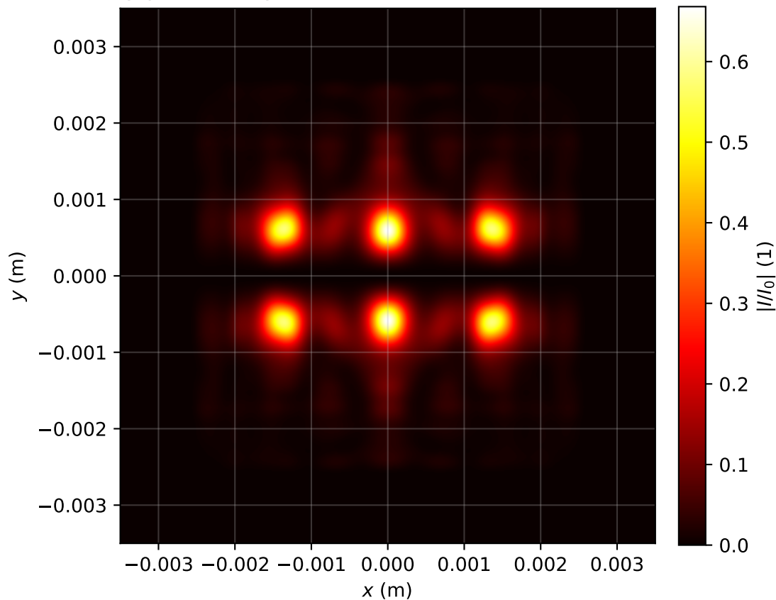
Intensity profile I(x, y, z = 2.946)/I_0 , P_{in}=5.0P_{cr} , artificial time
